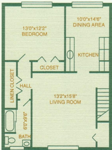
TYPICAL ONE BEDROOM SECOND FLOOR PLAN
