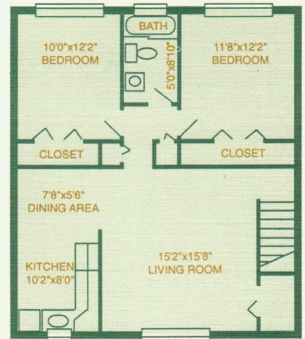
TYPICAL TWO BEDROOM SECOND FLOOR PLAN
