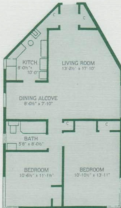
TWO BEDROOM
