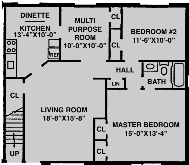
Large 2 Bedroom
